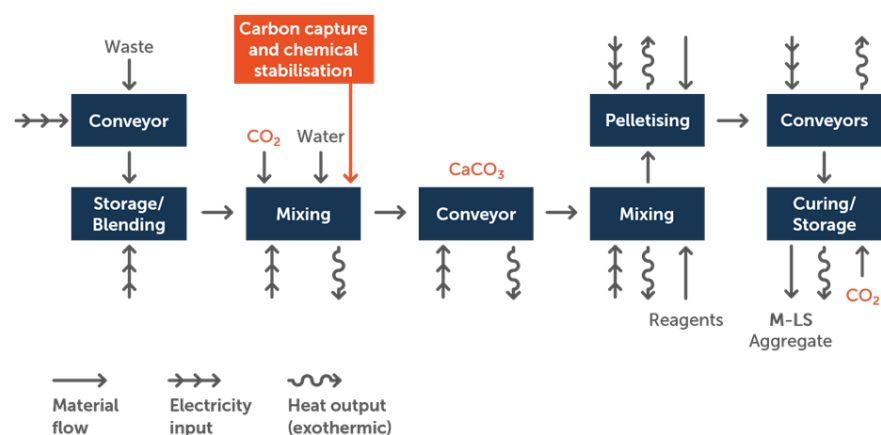
Figure 3: Manufacturing process
